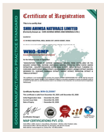
WHO - GMP
